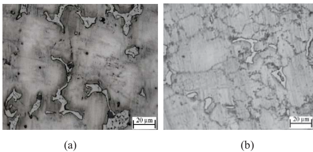
Fig. 2 Optical micrographs of as cast and forged MA alloy; (a) MA-cast and (b) MA-forged
