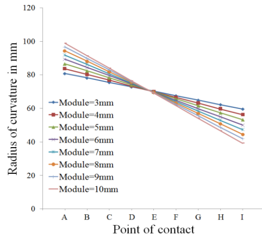
Figure 3. Variation of radius of curvature of gear tooth along path of contact [pressure angle 14.5^\circ ]
