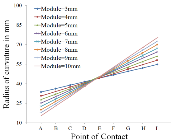
Figure 2. Variation of radius of curvature of pinion tooth along path of contact [ \phi=14.5^\circ ]
