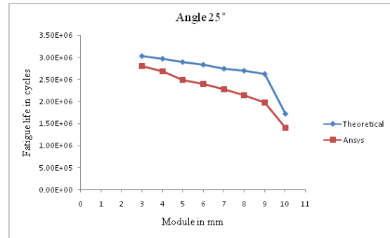
Figure 9. Fatigue life V/s Module at pressure angle 25°
