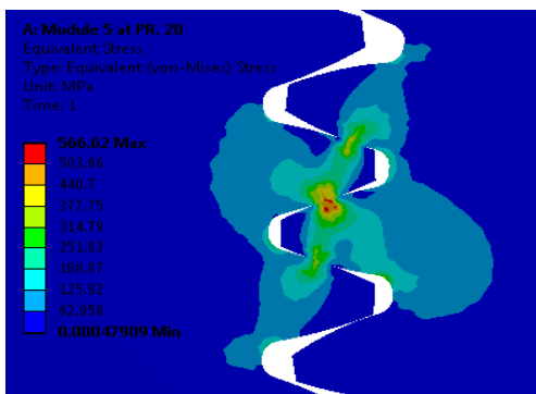
Figure 7. Von-mises stress for gear pair with module 5 and pressure angle 20°
