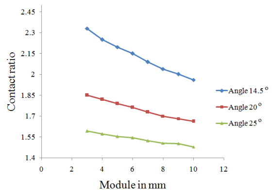
Figure 4. Contact ratio V/s Module for different pressure angles
