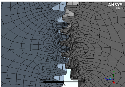
Figure 6. Hex-dominant meshing
