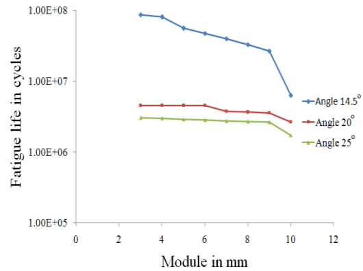
Figure 8. Fatigue life V/s Module for different pressure angles
