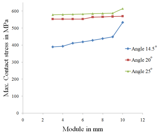
Figure 5. Max.Contact stress V/s Module for different pressure angles
