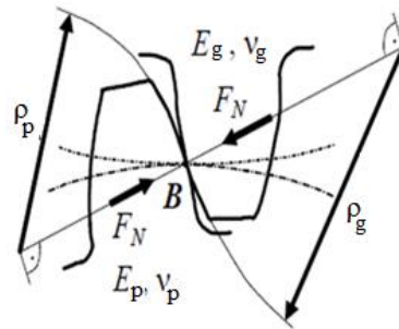
Figure 1. Contact between involute teeth
